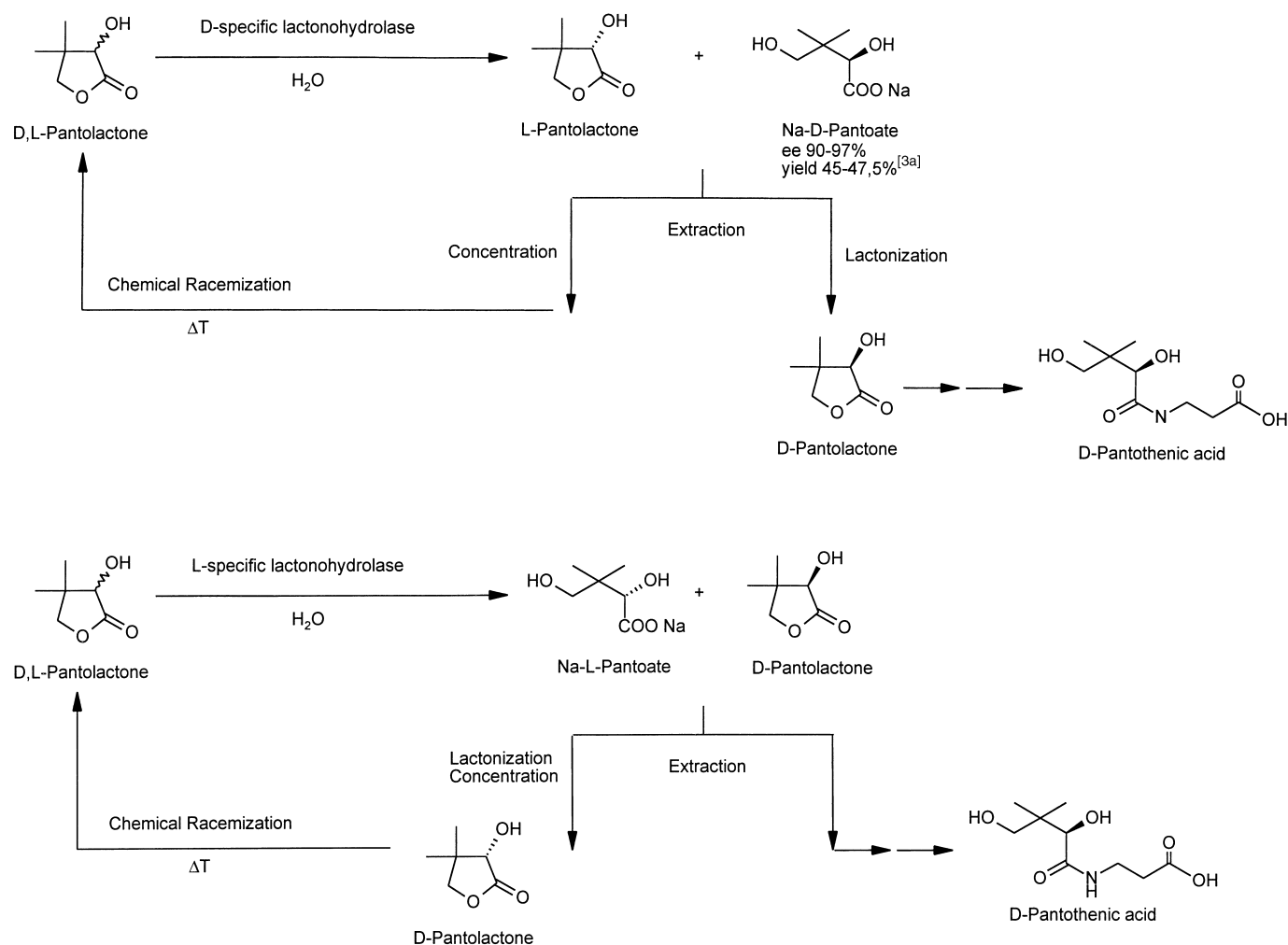
Figure 1. Production of D-pantothenic acid via resolution of D,L-pantolactone by either a D- or an L-specific lactonohydrolase.
